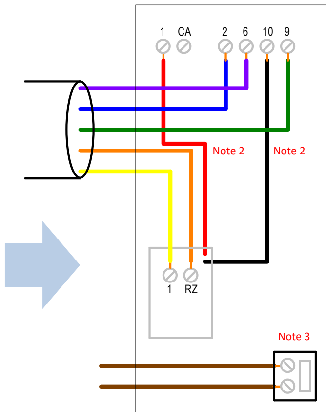
Urmet 1130/11 Handset
